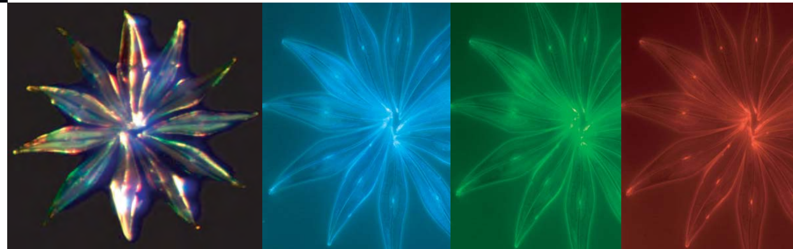
The diatom frustule is predominantly glass. In particular diatom species, the spacing of small features can facilitate the interaction with light. An example of refraction (left) and other three images taken with colored filters. Images of diatoms taken with a light microscope
