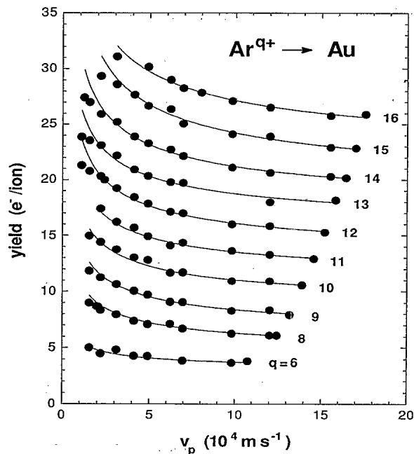
FIG. 2. Total electron yields vs impact velocity as derived from the measured ES, for impact of \text{Ar}^{q+} on clean polycrystalline gold ( q=6-16 ). The solid lines are fits according to Eq. (2). Note the clear deviation from these fits at low v_p which is ascribed to image-charge acceleration of projectiles.
