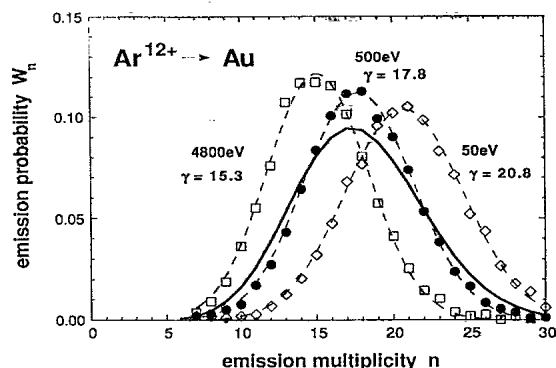
FIG. 3. Electron emission statistics (ES) as derived by unfolding the raw pulse height spectra (cf. Fig. 1) for impact of \text{Ar}^{12+} with different impact energies on clean polycrystalline gold. The dashed lines are fitted Gaussian distributions. For the 500-eV data a Poissonian (solid line) with appropriate mean value \gamma has been added (for further explanations see text).
