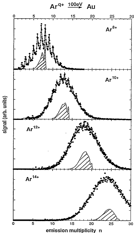
FIG. 1. Measured pulse height spectra for impact of 100-eV \text{Ar}^{q+} in different charge states on clean polycrystalline gold. Measured data were fitted (solid line) for deconvolution into individual multiplicities. The hatched insets show the energy deposition distribution for the respective most probable number of emitted electrons.
